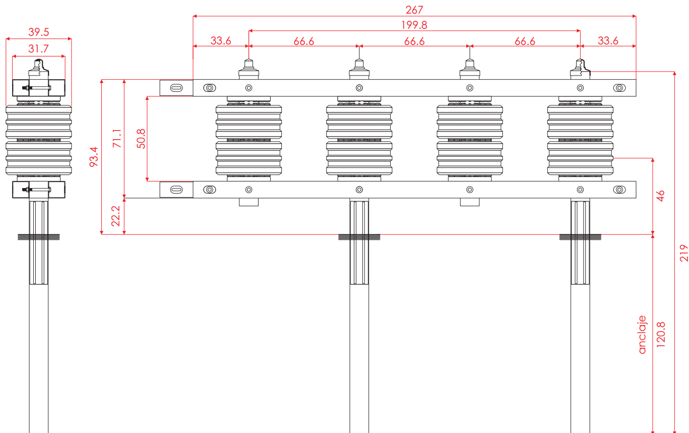
VISTA FRONTAL
